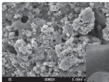
F-MELT® (×10,000)
